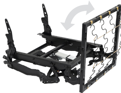
3508 Two-Motor Mechanism
